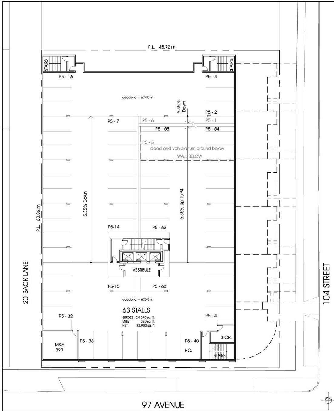
P5 / 2nd Level Below Grade
