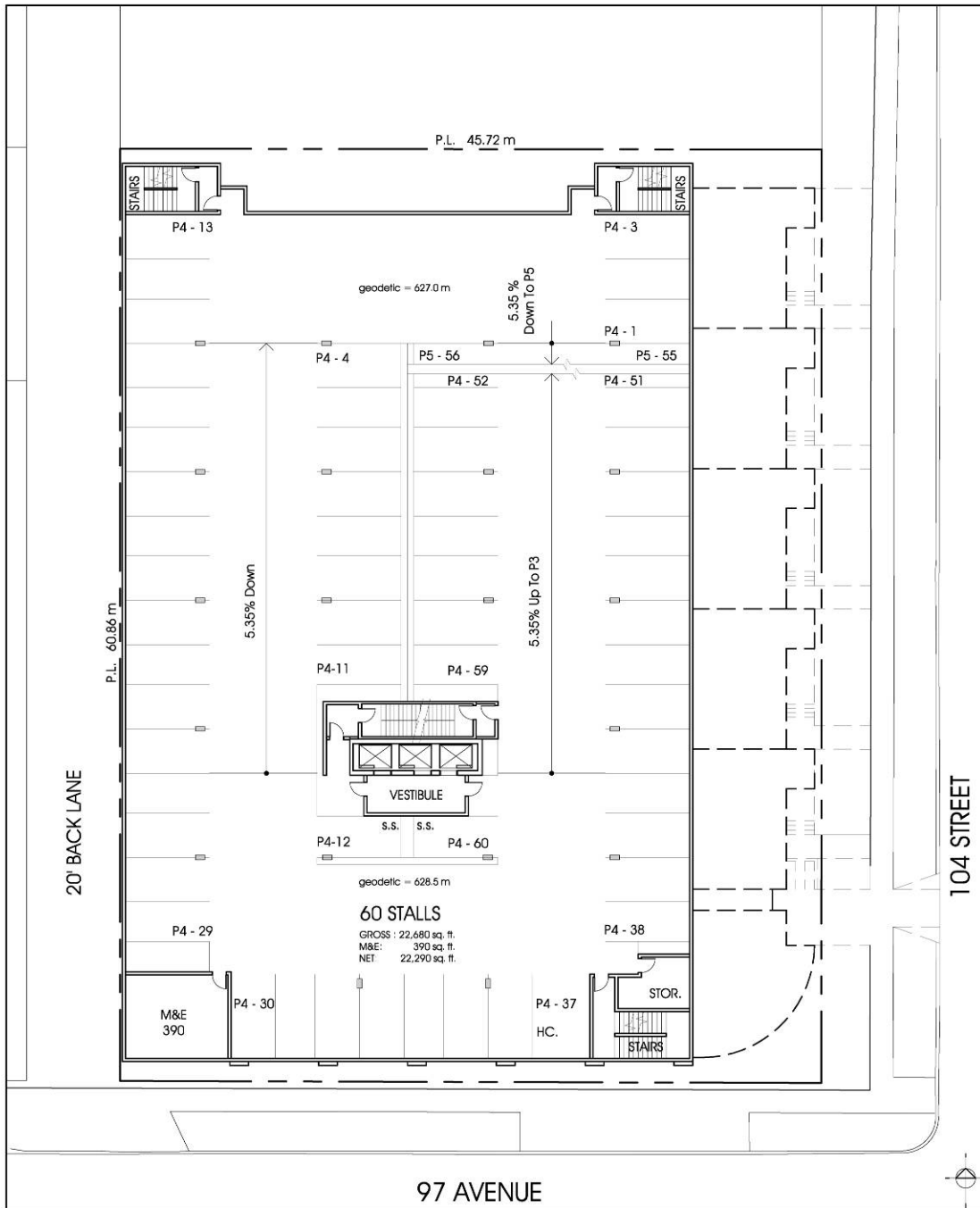
P4 / 1st Level Below Grade
