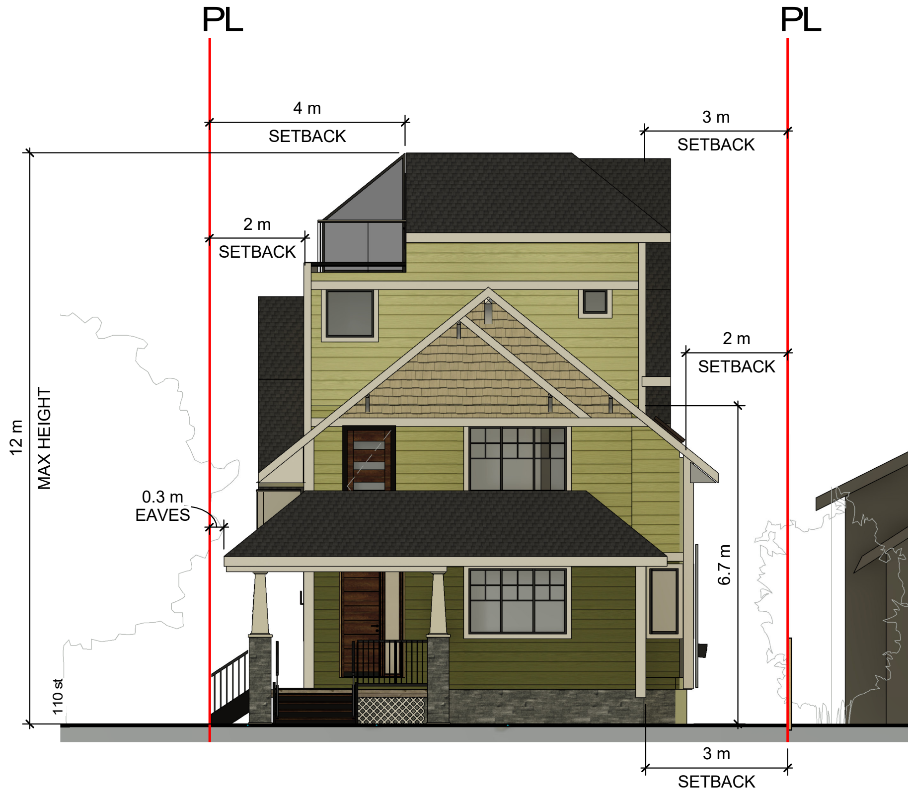
APPENDIX 2c SOUTH ELEVATION
