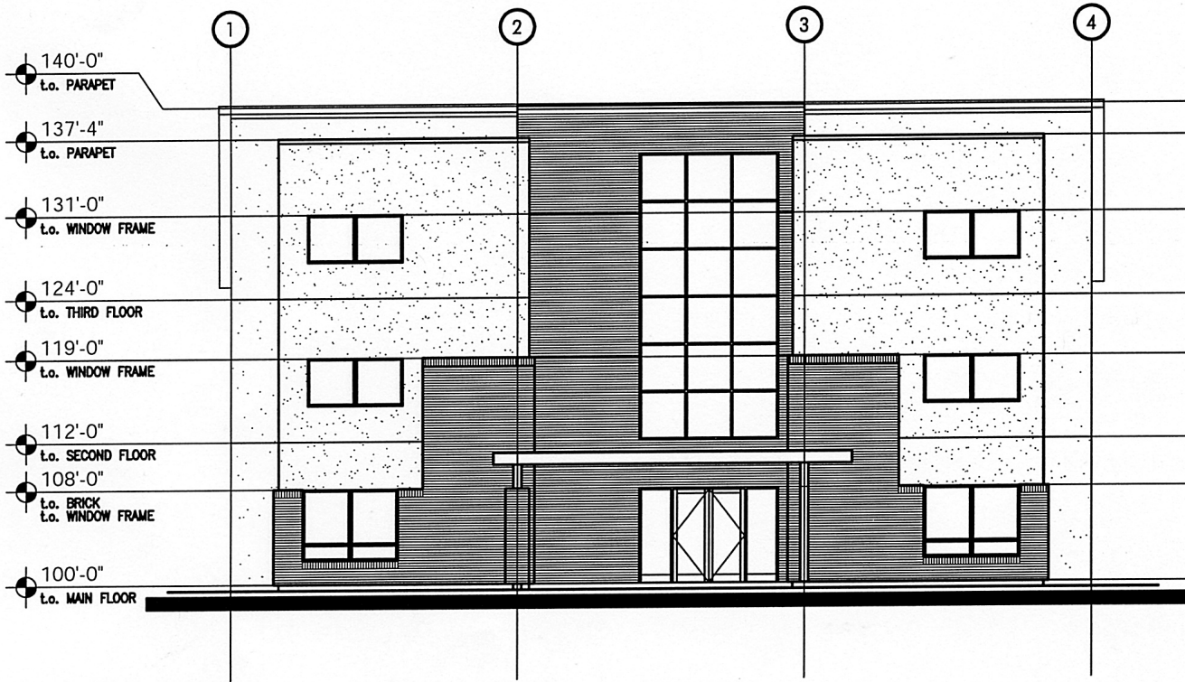
NORTH ELEVATION
