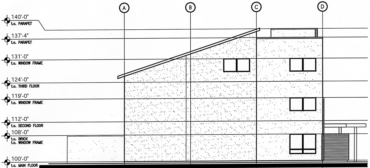
EAST ELEVATION
