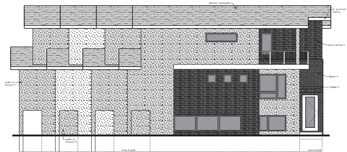
WEST ELEVATION
